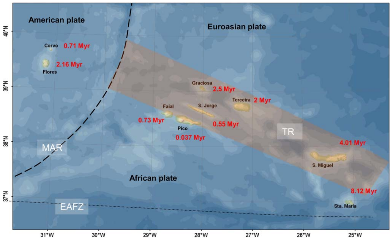
Fig. 1 Location of the Azores archipelago in the North-Atlantic Ocean and main tectonic features ( MAR Middle Atlantic Ridge, TR Terceira Rift, EAFZ East Azores Fracture Zone). Maximum age for inland outcrops is presented
